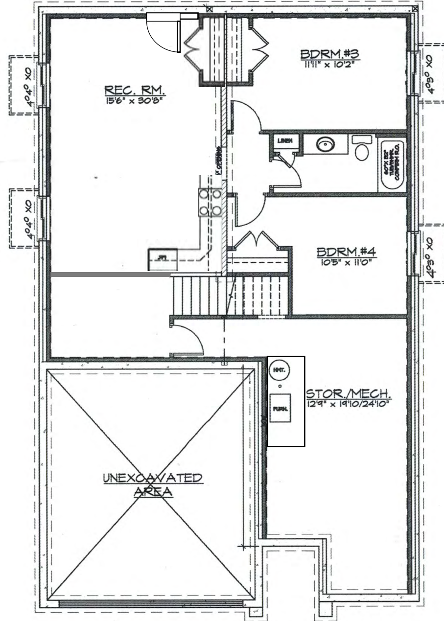
BASMENT FLOOR PLAN FINISHED AREA = 905 SQ. FT. STOR./MECH. 374 SQ. FT. (INCLUDING UNDER STAIRS)
