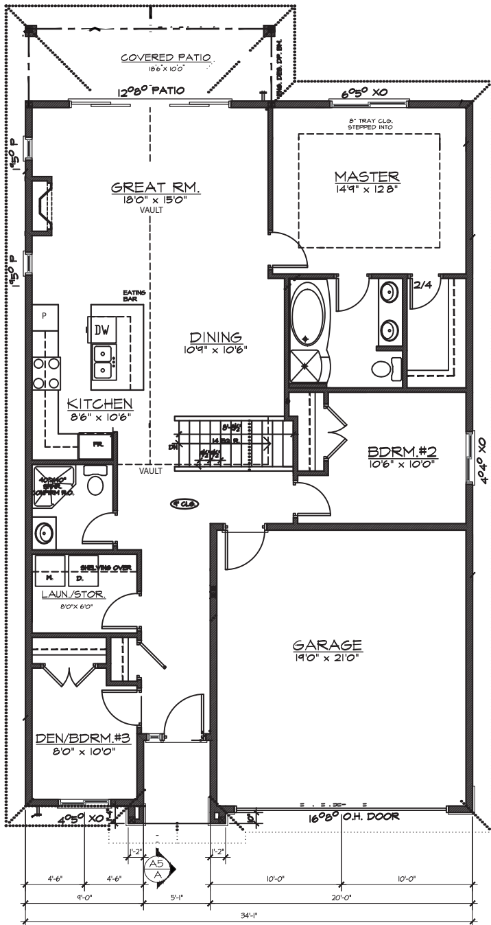
MAIN FLOOR PLAN FINISHED AREA = 1393 SQ. FT. (9' CEILING)
