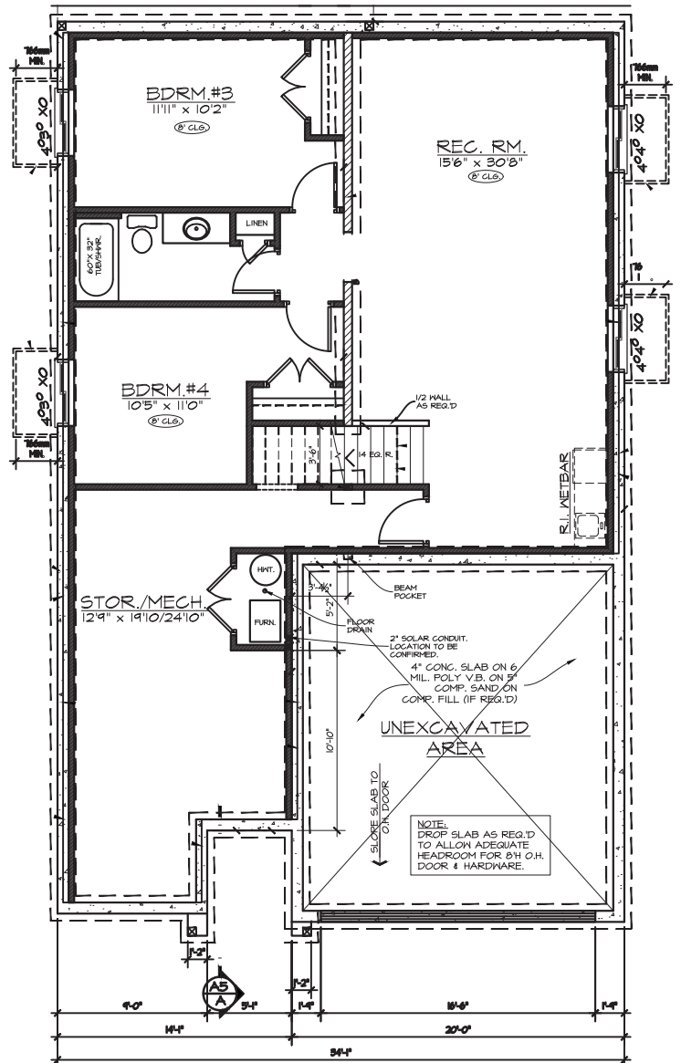
BASMENT FLOOR PLAN FINISHED AREA = 905 SQ. FT. STOR./MECH. 374 SQ. FT. (INCLUDING UNDER STAIRS) (8' CEILING)
